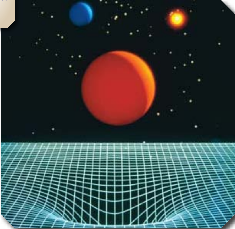
This illustration shows how an object's gravity curves space.
